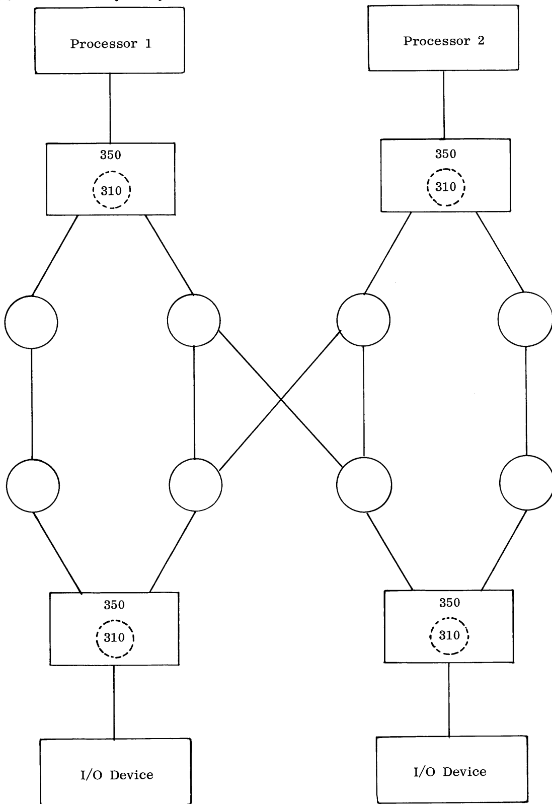
Figure 2-3 is an example only and illustrates a 2 x 2 switching complex.
