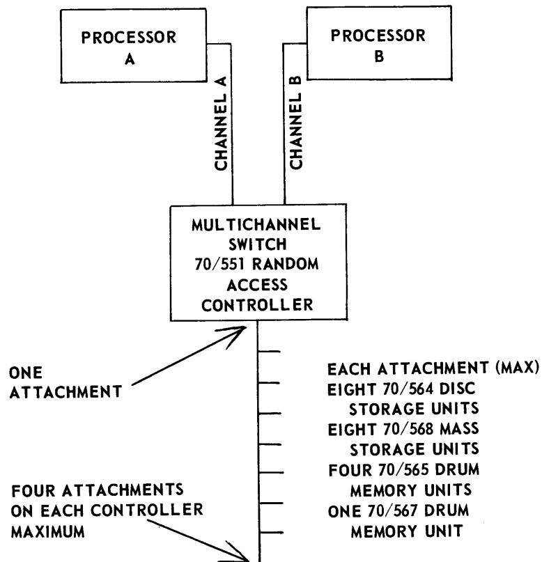
Figure 2-4. Multichannel Switch
